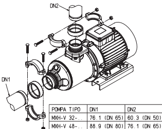
Bocche con giunti Victaulic Victaulic ports Victaulic-Anschlüsse Raccords Victaulic Acoplamiento Victaulic 进出口卡箍
